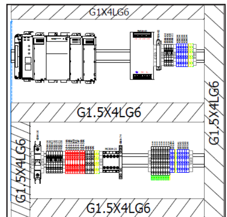
Transfer Panel
