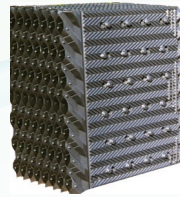
Opti-Pac 7500 Fill Crossflow Fill Integrated Louver and Drift Eliminator (Bottom supported crossflow fill packs replace OEM Hanging Sheets)
